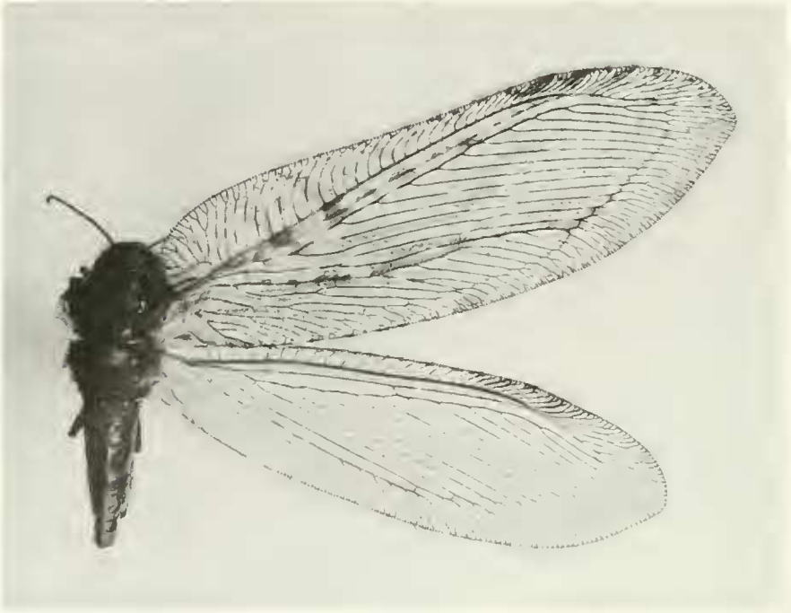
Fig. 6. Polystoechotes gazullai , female, body and wings.
